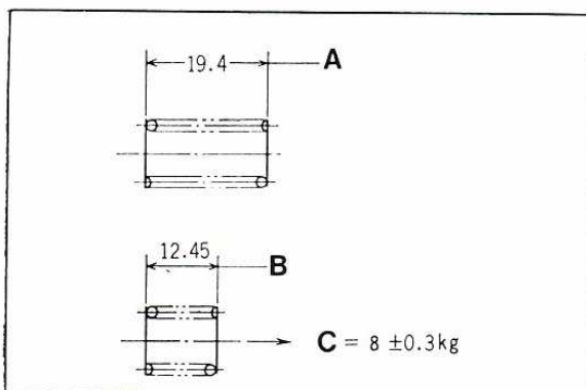
Fig. 60. — RESSORT DE SOUPAPE.
